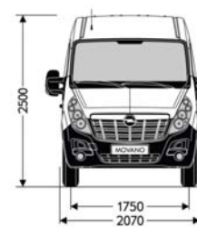
Opel Movano Crew Van FWD L2H2
