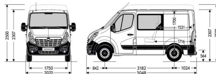
Opel Movano Crew Van FWD L1H1-H2
